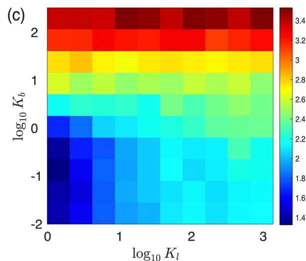
Fig. 7 (a) The offset k obtained from fits of the area flow rate Q(w) to eqn (1) versus E_{sp} (with \theta_w = 90^\circ ) using the 2D SP model in the \lambda \rightarrow \infty limit (stars) and \lambda \rightarrow 0 limit (circles). The offset k for the 2D frictionless DP model on a color scale (b) from 0 (blue) to 1.7 (red) in the \lambda \rightarrow 0 limit (with \theta_w = 90^\circ ) and (c) from 1 (blue) to 3.5 (red) in the \lambda \rightarrow \infty limit (with \theta_w = 90^\circ ) as a function of the perimeter K_t and bending K_b energy scales.
